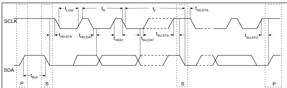
FIGURE 10.3 – SmBus TIMING
